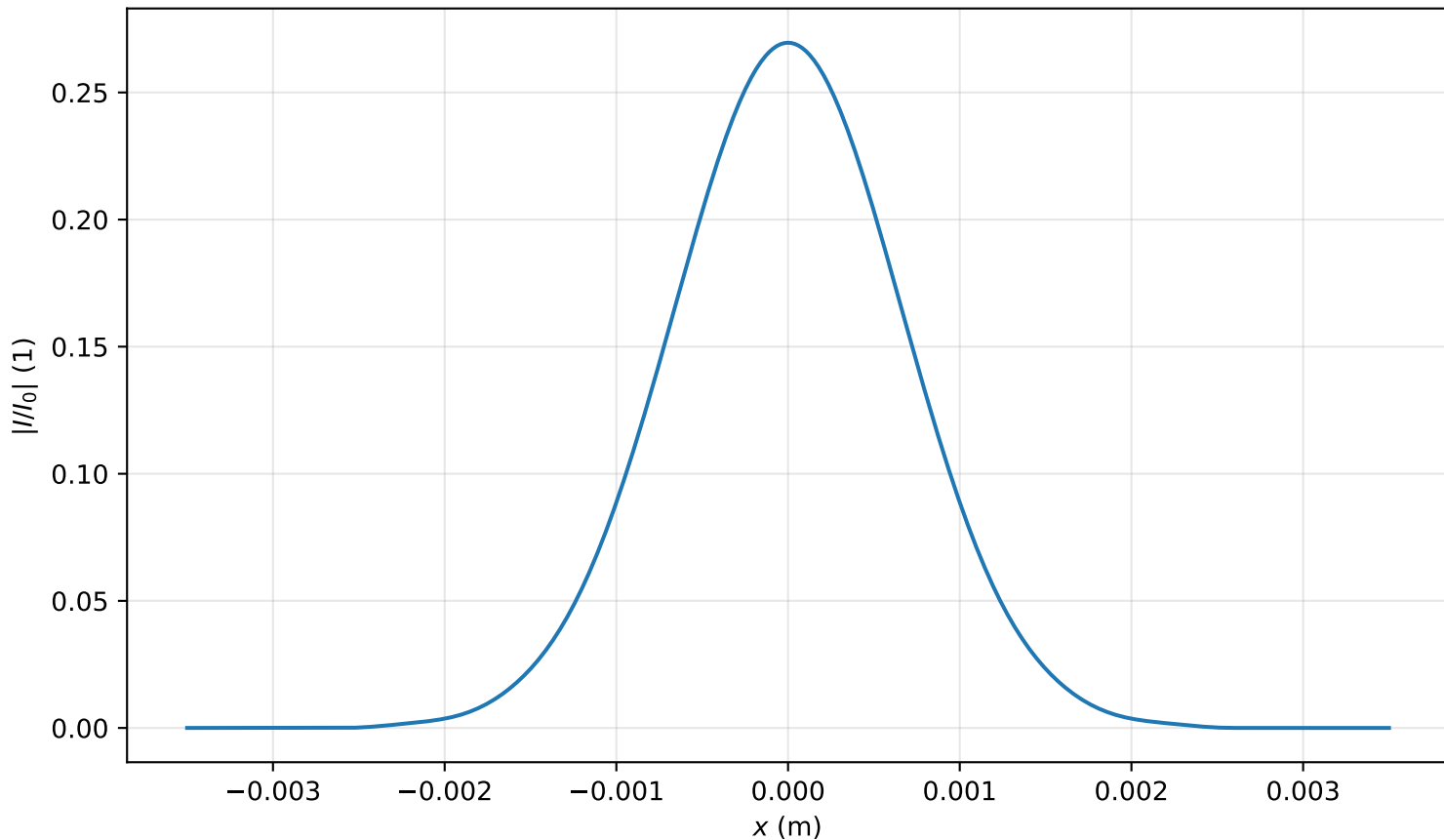
Intensity profile I(x, y = 0, z = 3.503m)/I_0 , P_{in}=0.1P_{cr} , artificial time
